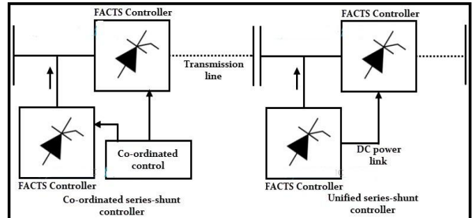
Fig. 4. Combined Series Shunt Controllers
