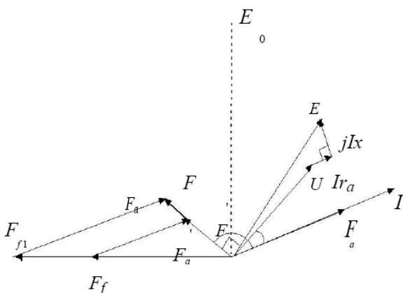
Figure 2. Magnetic-electronic potential vector of generators considering saturation
