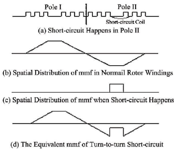
Figure 1. Spatial distribution of mmf in rotor windings
