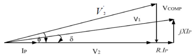
Fig-4 Phasor diagram with series compensation phasor diagram of Fig-4, VCOMP generates a voltage with opposite direction to the voltage drop in the line inductance because it lags the current I_P [3].
