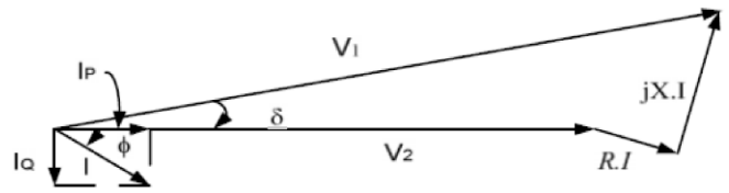
Fig-2 Phasor diagram without compensation
