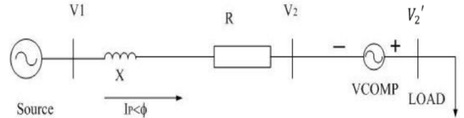
Fig-3 Representation of AC system with series compensation
