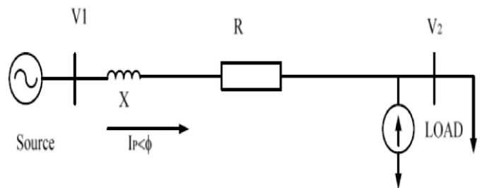
Fig-5 Representation of AC system with Shunt compensation
