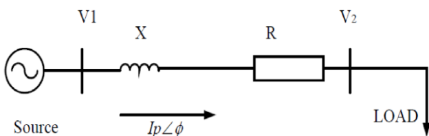
Fig-1 Representation of AC system
