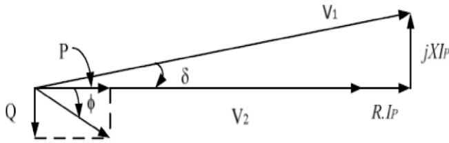
Fig-6 Phasor diagram of AC system with shunt compensation. The shunt capacitive compensator is used to improve the power factor, most of the practical loads are inductive and results into lagging power factor. To compensate, a shunt capacitor is connected which draws current leading the source voltage. The net result is improvement in power factor. The shunt inductive compensator is used either when charging the transmission line, or, when there is very low load at the receiving end. To compensate, shunt inductors are connected across the transmission line. In Fig-5, a current source device is being used to compensate the reactive component of the load current (IQ). As a result, the system voltage regulation is improved and the reactive current component from the source is reduced or almost eliminated as shown in Fig-6. Also a current source or a voltage source can be used for inductive shunt compensation[3].
