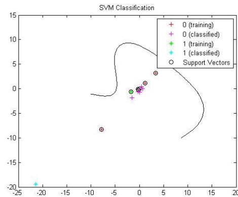
The above picture demonstrate the SVM classification of EEG signals.
