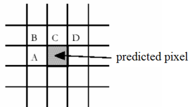
Fig. 1. Predictor Model
