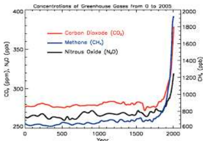
Chart.1. Concentration of Greenhouse Gases over the years
