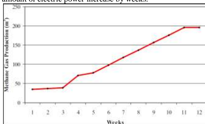
Fig.5. The amount of methane gas produced per week
