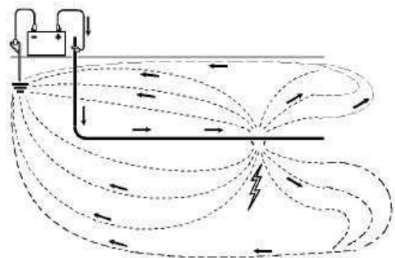
Figure 1 An A-Frame method of finding cable fault location
