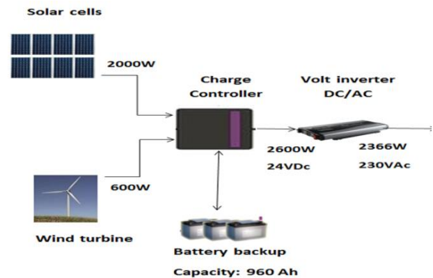
Fig 1.1: Block diagram of hybrid system
