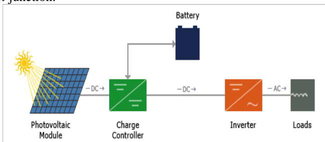
Fig 3.1: Actual understanding of PV system
