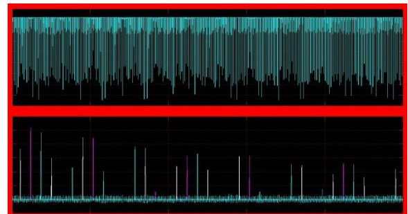
Fig5.10: Three phase VI measurement (Hybrid+battery)
