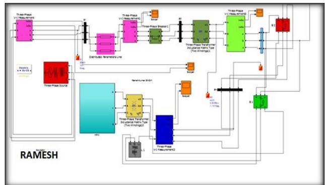
Fig 5.1 Basic Layout
