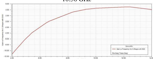
Fig.8 Gain V/s Frequency of rectangular slot patch antenna
