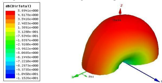
Fig.10 3D Polar plot of rectangular slot patch antenna at 10.36 GHz
