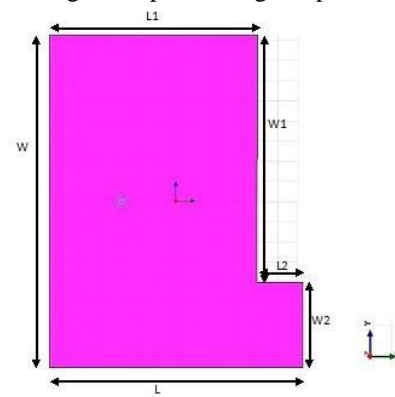
Fig.2 L- Shaped patch
