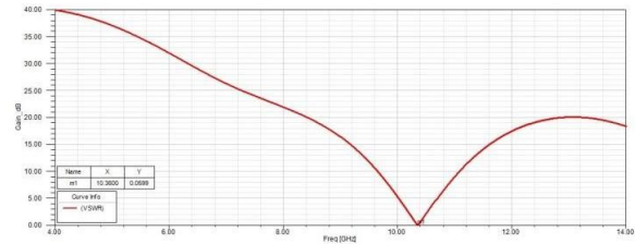
Fig.9 VSWR of rectangular slot patch antenna
