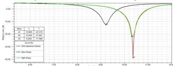
Fig.5 Return loss plot for base shape, L-Shaped
