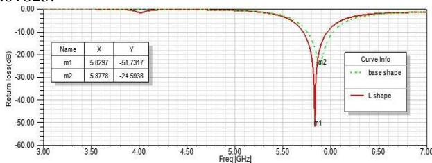
Fig.4 Return loss and bandwidth plot
