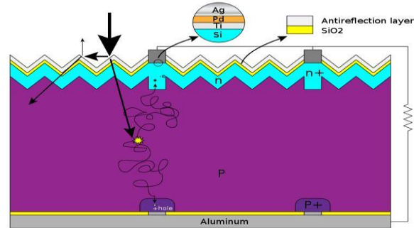
Fig(1): Silicon_Solar_cell_structure
