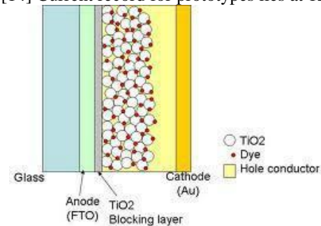
Fig(2): dye-sensitized solar cell
