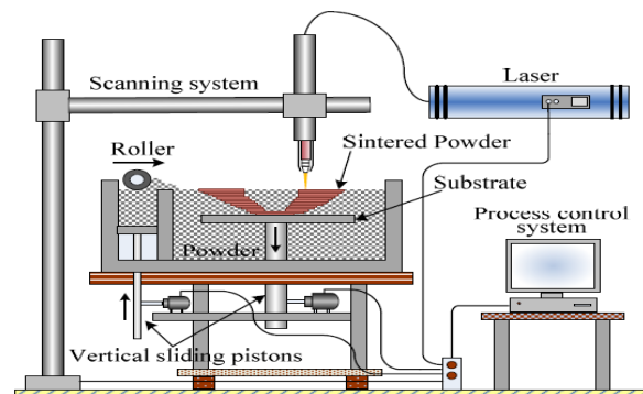
Fig.2: Schematic of Laser Sintering
