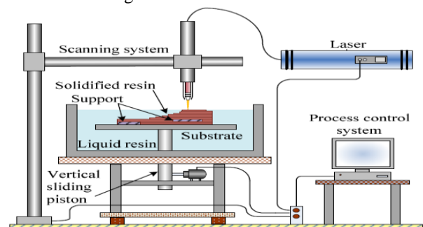
Fig.1 (Schematic of stereolithography)
