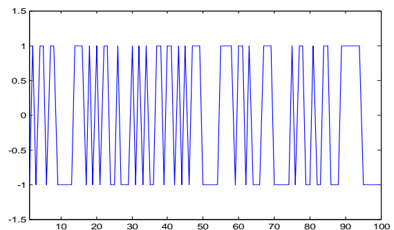
Figure 12: Initial 100 samples of BPSK modulated binary data.
