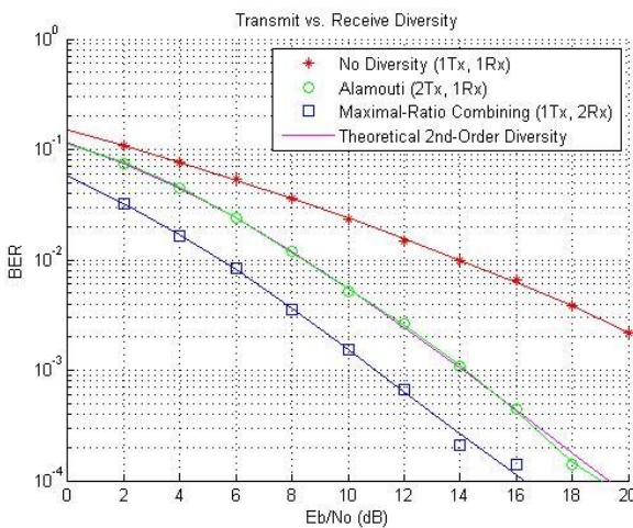
Figure 9: BER performance at different MIMO coding schemes for 1x2 or 2x1 systems.
