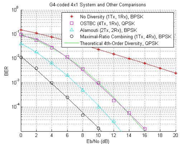
Figure 10: BER performance at different MIMO coding schemes for higher order diversity.
