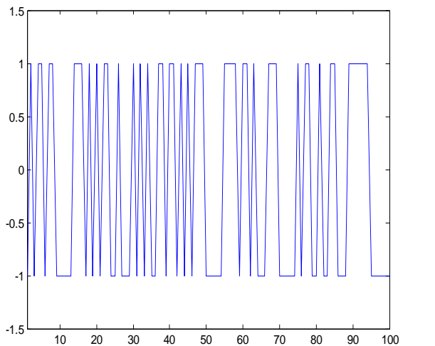
Figure 8 : Initial 100 samples of BPSK modulated binary data.
