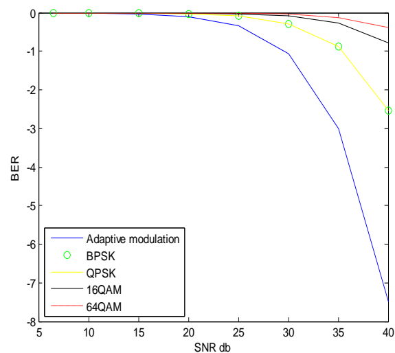
Figure 7 : Performance evaluation of CP based channel estimation and correction in terms of BER at different modulation for MIMO OFDM systems.
