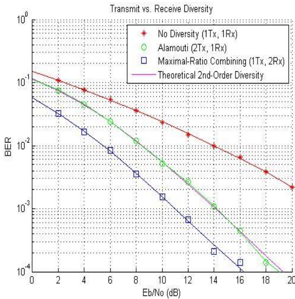
Figure 5 BER performance at different MIMO coding schemes for 1x2 or 2x1 systems.
