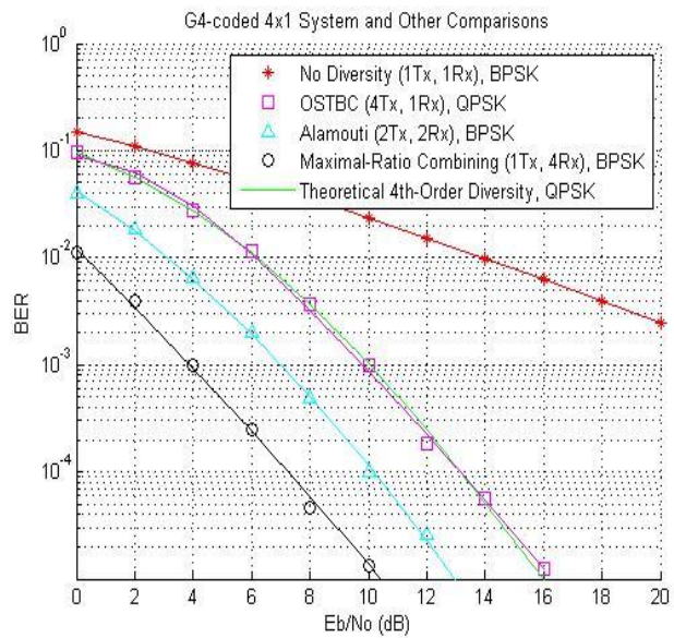
Figure 6: BER performance at different MIMO coding schemes for higher order diversity.
