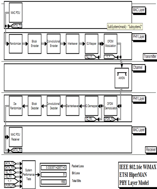
Figure 1: Simulink model for Wi-Max Physical layer without fading
