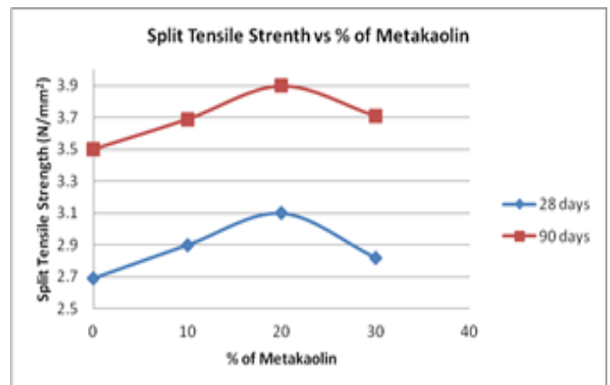
Figure 3 Graph between Split Tensile Strength of concrete for M20 vs % of metakaolin
