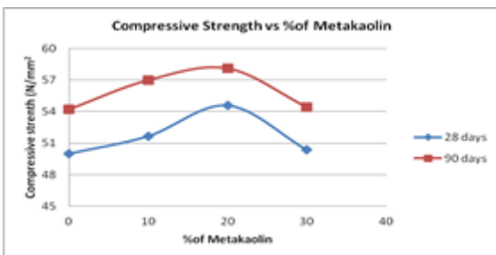
Figure 1 Graph between Compressive Strength of concrete for M20 vs % of metakaolin
