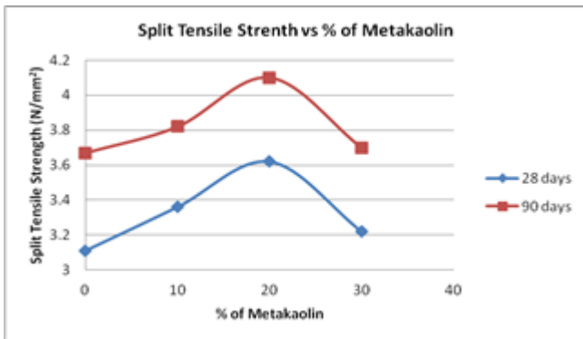
Figure 4 Graph between Split Tensile Strength of concrete for M40 vs % of metakaolin
