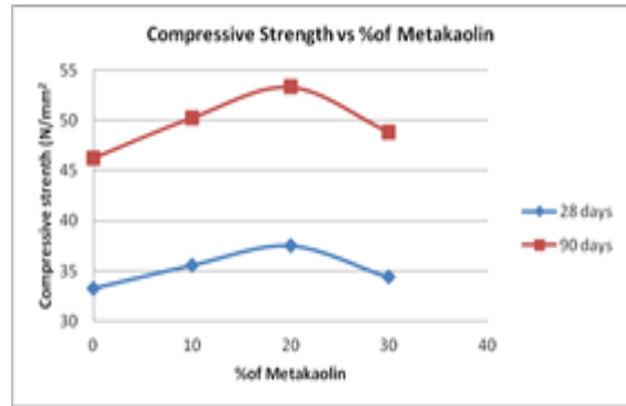
Figure 2 Graph between Compressive Strength of concrete for M40 vs % of metakaolin
