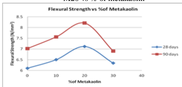
Figure 6 Graph between Flexural Strength of concrete for M20 vs % of metakaolin
