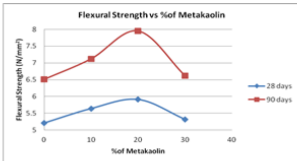
Figure 5 Graph between Flexural Strength of concrete for M20 vs % of metakaolin
