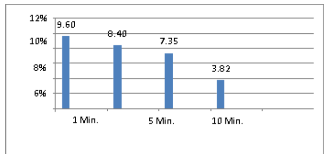
Figure 1 - Water absorption % after abrasion of RA
