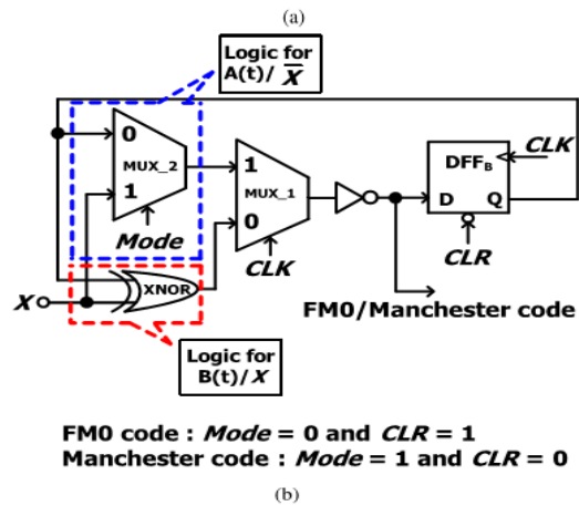
Fig. 12. VLSI architecture of FM0 and Manchester encodings using SOLS technique. (a) Unbalance computation time between A(t)/X and B(t)/X. (b) Balance computation time between A(t)/X and B(t)/X.
