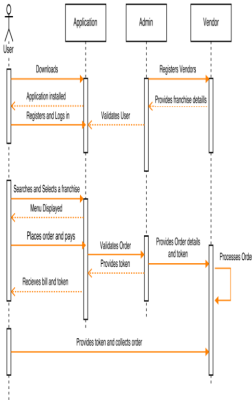
Figure 2. Sequence Diagram
