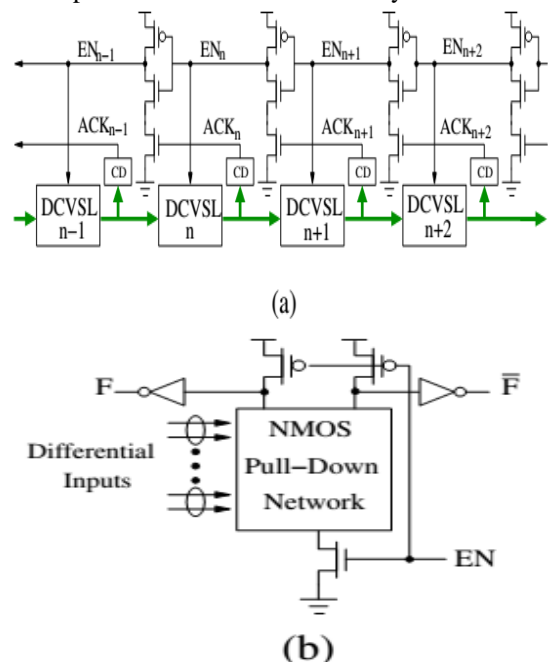
Fig. 1. (a) Zero-delay-overhead self-timed pipeline structure, and (b) DCVSL structure.
