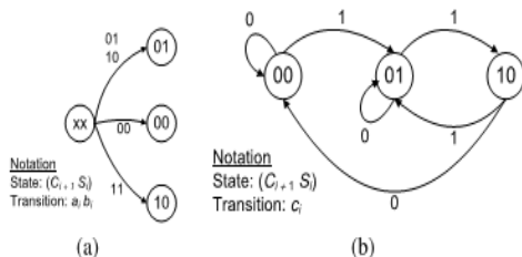
Fig. 3. State diagrams for PASTA. (a) Initial phase. (b) Iterative phase
