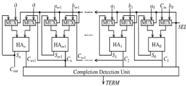
Fig. 2. General block diagram of PASTA
