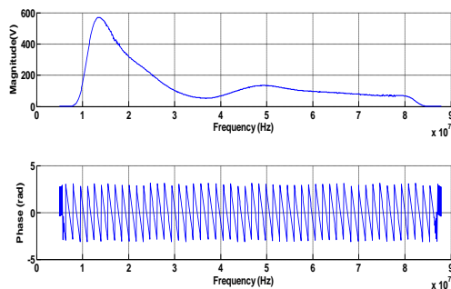
Figure 16: Channel Estimate
