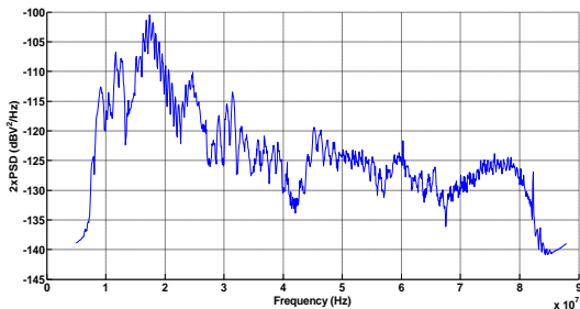
Figure 13: PSD of Noise
