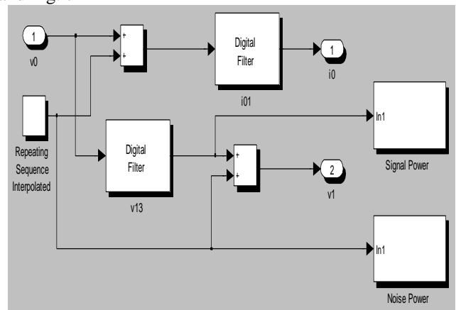
Figure 5: PLC line model with noise measured
