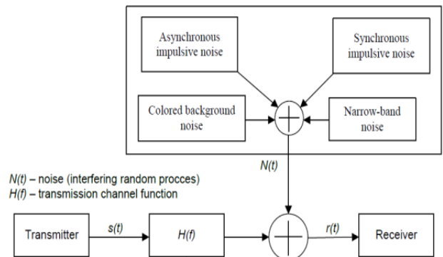
Figure 4: PLC channel model.
