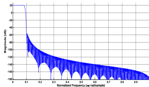
Figure 12: Response of FIR Interpolation Filter
