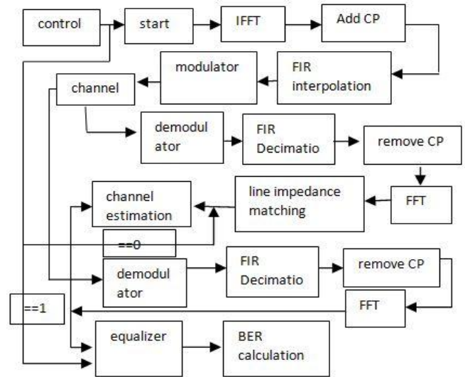
Figure 1: Block diagram of PLC Channel and Impedance estimation model.
