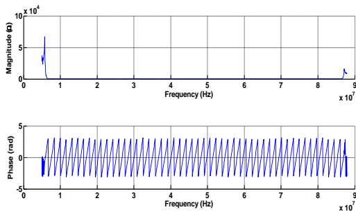
Figure 14: Transmitter Impedance
