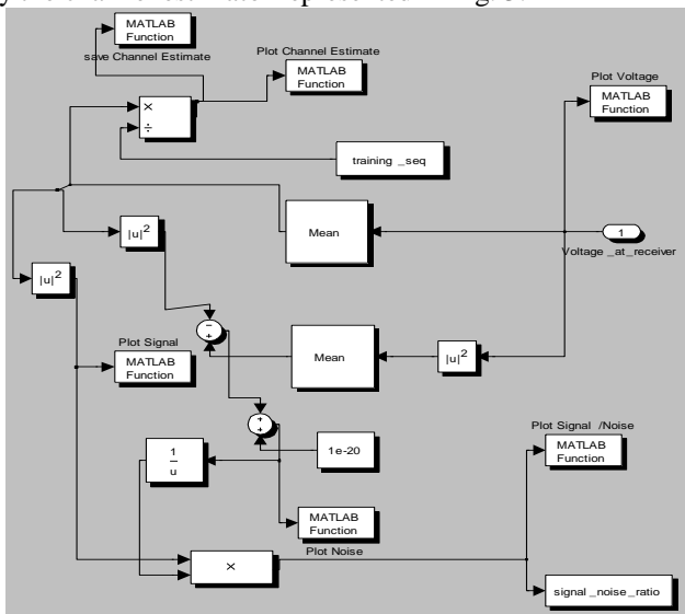
Figure 3: The block diagram of channel estimation The channel estimation block is responsible of estimating the channel taps and estimating the SNR on each sub-carrier. The estimation of the channel taps is done simply by doing a division between the known training sequence and the corresponding received sequence, since we work here in the frequency domain. For the SNRs estimation, we are obligate to work in each sub-carrier trying to separate the noise from the desired signal, and compute the power of desired signal divided by the power of the estimated noise. When we obtain these SNRs, they will be sent back to the transmitter and saved at the receiver for the next use, which choose the
