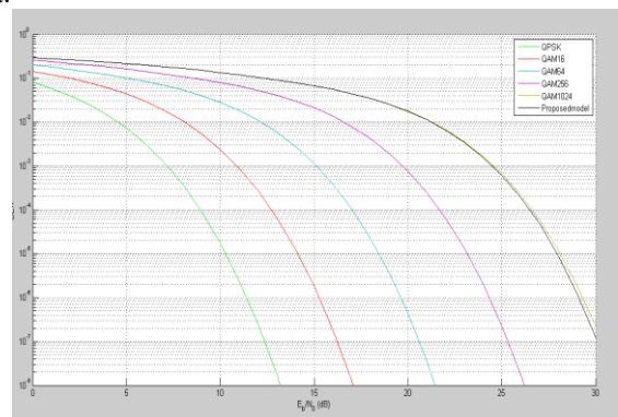
Figure 18: BER dependence on Eb/N0 for particular modulation in OFDM system
