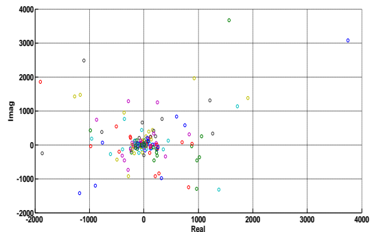
Figure 10: Transmitter Constellation diagram for 1024-QAM
