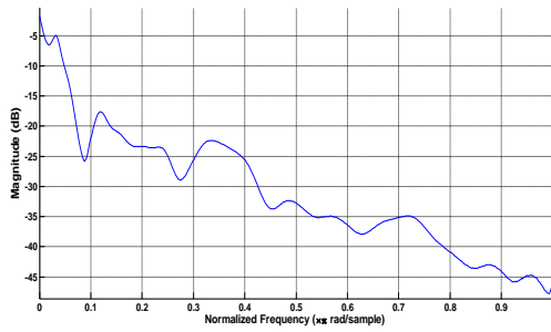
Figure 6: Magnitude Response of Digital Filter
