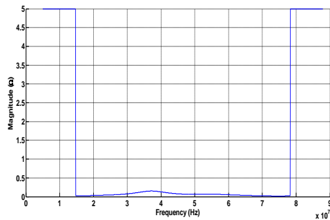
Figure 15: Receiver Impedance
