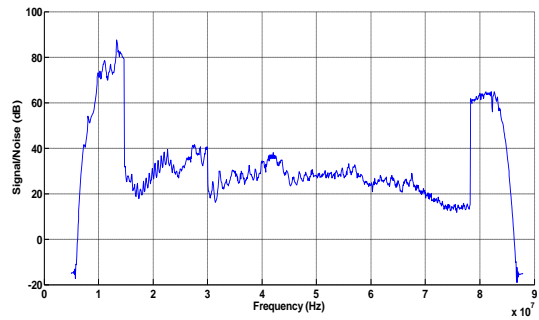
Figure 17: Signal/Noise ratio
