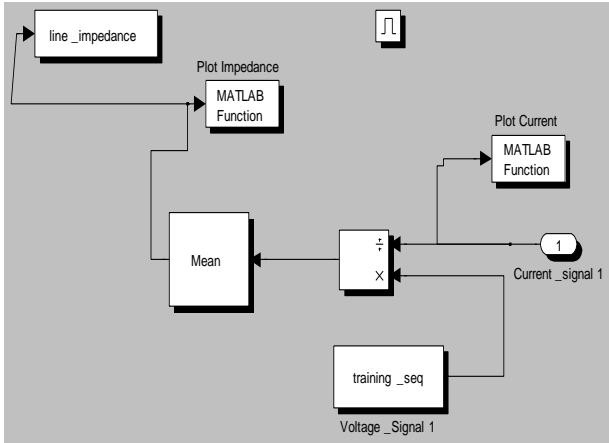
Figure 2: The block diagram of impedance estimation For the second channel use, the impedance estimator will be disabled and the channel estimator block and the equalizer block can work normally starting from this second channel use until the end of the connection. In this time, the signal contains information data and a small training sequence used by the channel estimator represented in Fig. 3.
