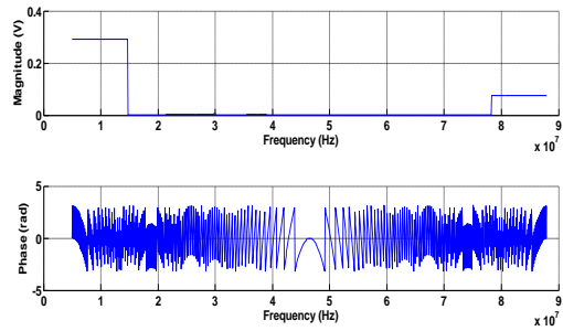
Figure 9: Training sequence
