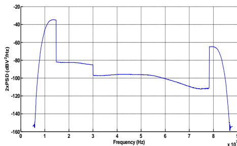
Figure 8: Transmitted signal
