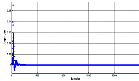
Figure 7: Impulse response of Digital Filter
