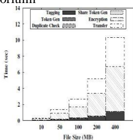
Fig. 2. Time Breakdown for Different File Size
