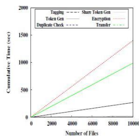
Fig. 3. Time Breakdown for Different Number of Stored Files
