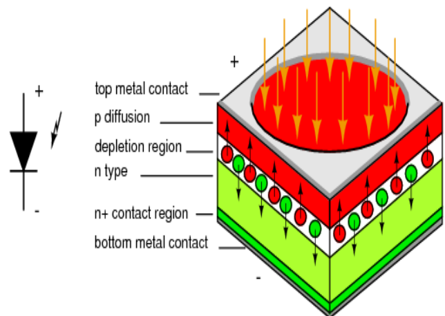
Figure 6: Avalanche photo diode
