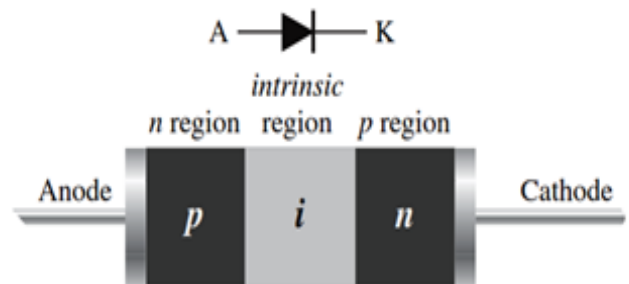
Figure 5: Pin diode
