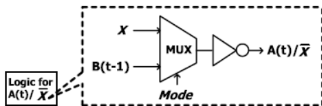
Fig. 7 Balance logic-operation sharing of A(t) and X.
