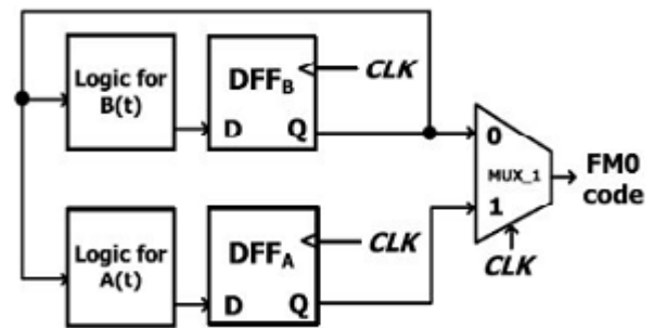
Fig. 5. FMO encoding with Area compact retiming
