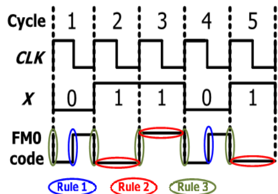
Fig. 2 Illustration of FM0 coding example
