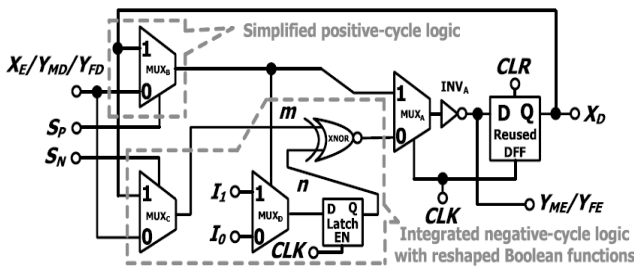
Proposed VLSI hardware architecture of FM0/Manchester codec
