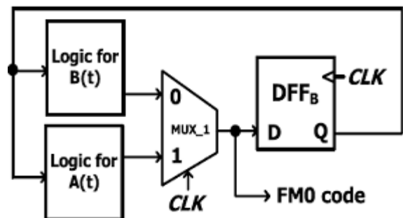
Fig. 6.FMO encoding without area compact retiming
