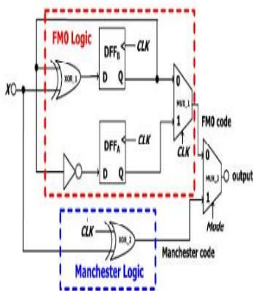
Fig. 4 Hardware architecture of Fm0/Manchester Code The active components means the components are work in the both fm0 and Manchester code. The total components means the number of the components are present in the hole circuit. the HUR rate is given below the following section
