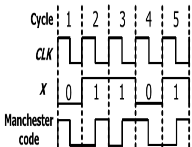
Fig. 3 Illustration of Manchester coding
