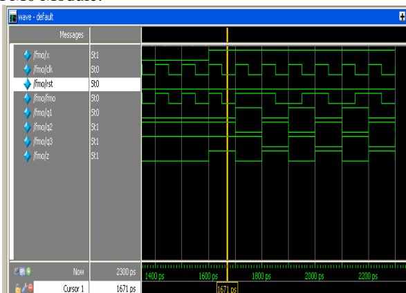
FM0 Code
