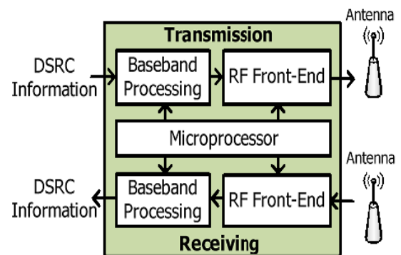
Fig. 1. System architecture of DSRC transceiver.
