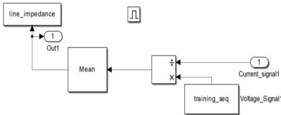
Figure 5: The block diagram of impedance estimation.
