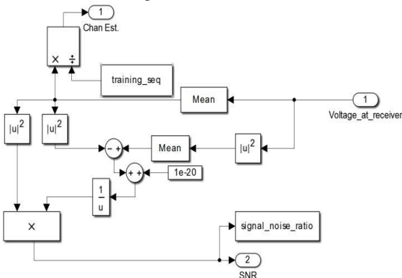
Figure 6: The block diagram of channel estimation
