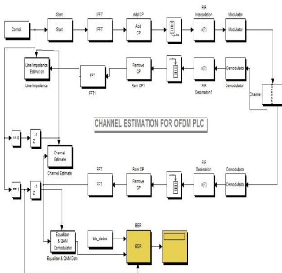
Figure 3: The Proposed OFDM based PLC network.
