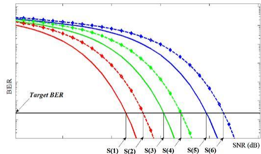
Figure 7: SNR thresholds selection for different mapping
