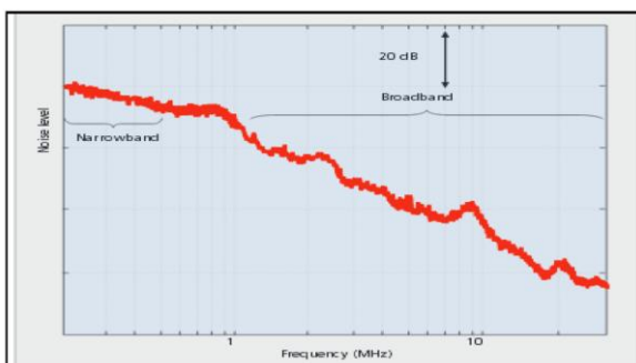
Fig 2- transfer characteristics of the power line channel
