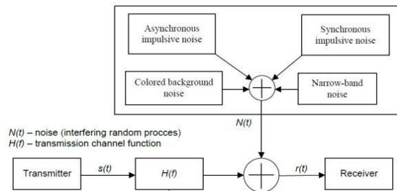
Figure 7: PLC channel model.
