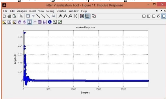
Figure 9: Impulse response of Digital Filter
