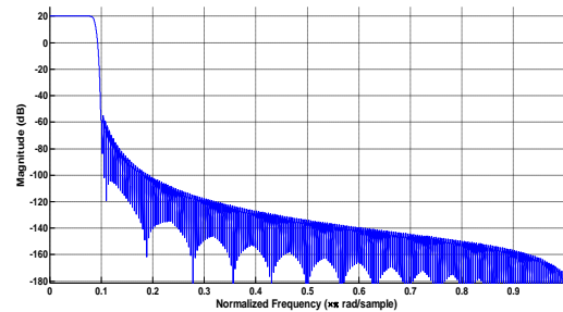
Figure 12: Response of FIR Interpolation Filter OFDM modulation gives good performance in communication channel with harsh characteristics. So the input coded data is modulated using OFDM modulation technique. The OFDM data is transmitted through the PLC channel which contains periodic impulsive noise. Fig.13 shows the PSD of noise.
