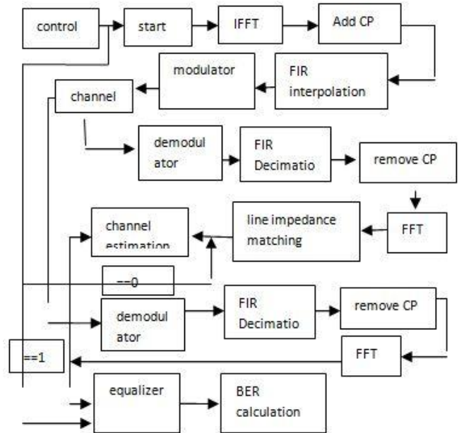
Figure 1: Block diagram of PLC Channel and Impedance estimation model.
