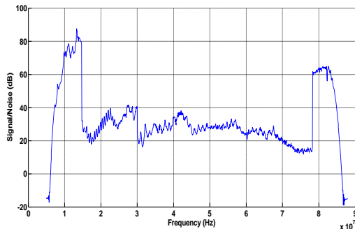
Figure 17: Signal/Noise ratio
