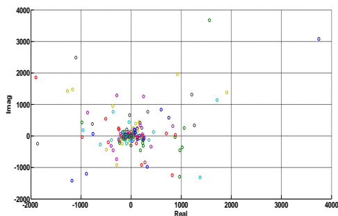
Figure 10: Transmitter Constellation diagram for 1024-QAM
