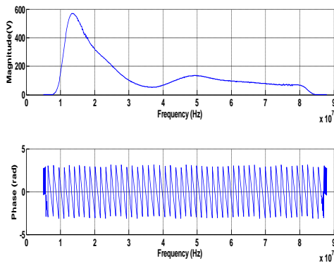
Figure 16: Channel Estimate
