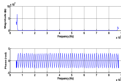
Figure 14: Transmitter Impedance
