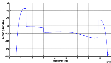
Figure 8: Transmitted signal
