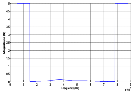
Figure 15: Receiver Impedance
