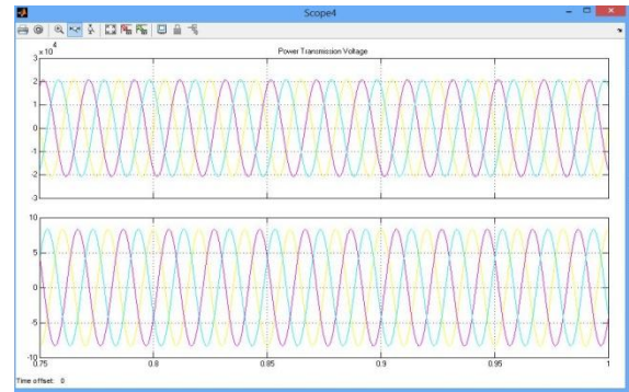
Fig 5.8: Output of Three-Phase V-I Measurement (Hybrid)
