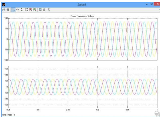
Fig 5.6: Output of Three-Phase V-I Measurement3 (Photovoltaic voltage for 1 month)
