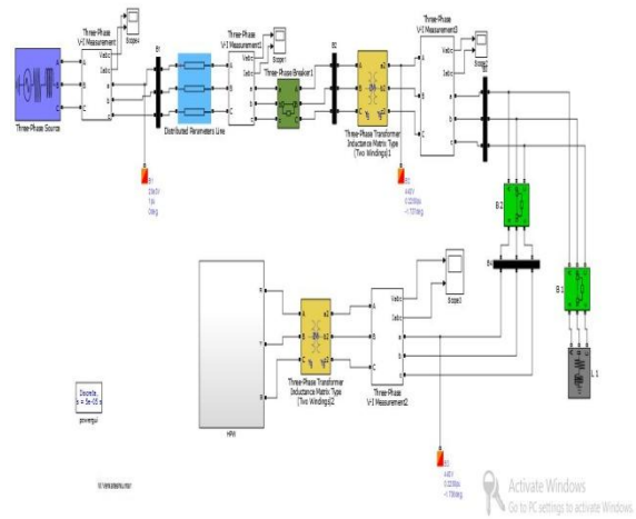
Fig 5.1 Basic Layout
