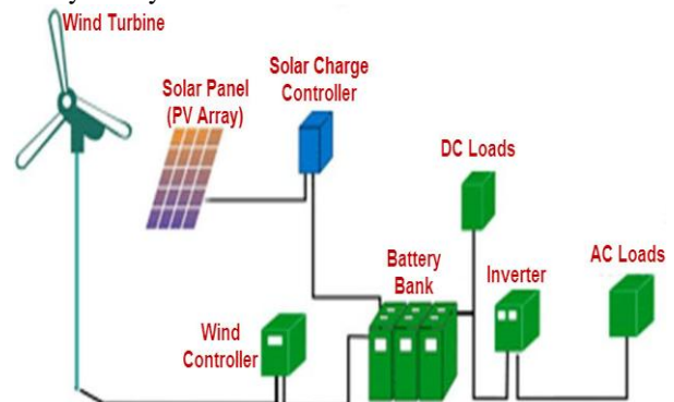
Fig 1.1: Block diagram of hybrid system
