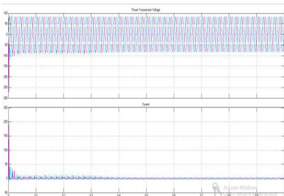
Fig 5.7: Output of Three-Phase V-I Measurement2-Current Measurement
