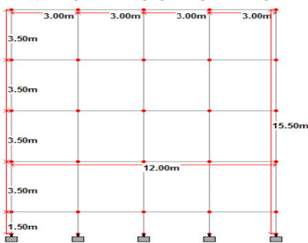
ELEVATION OF A SLOPING GROUND (0 DEGREE)
