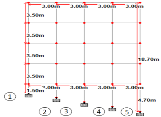
ELEVATION OF A SLOPING GROUND (15 DEGREE)
