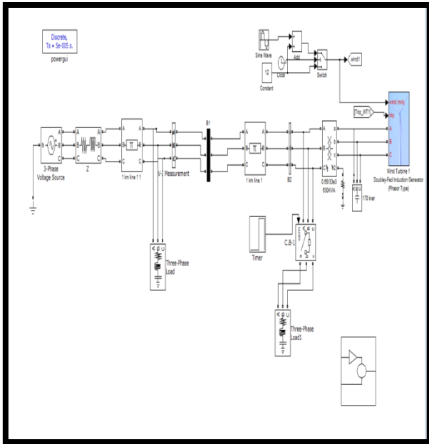
Fig 5.1- Single DFIG based Wind Power Plant
