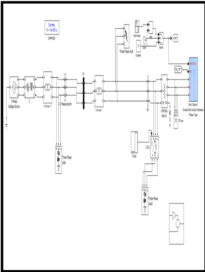
Fig 5.7- Proposed Matlab model with fault condition
