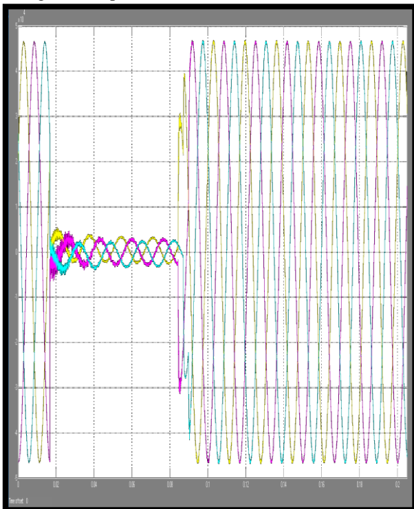
Fig 5.8- Voltage at B-1 during fault condition
