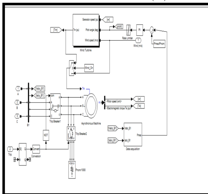
Fig 5.2- Subsystem of DFIG
