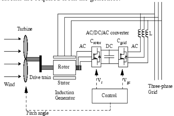
Fig-Operating Principle of the Wind Turbine Doubly-Fed Induction Generator
