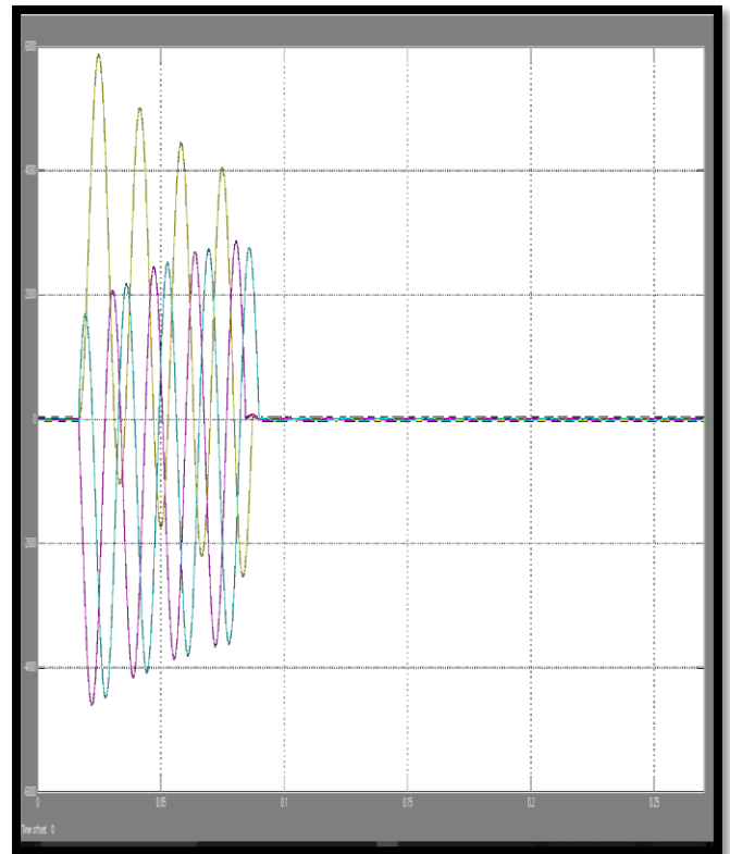
Fig 5.9 Current at B-1 during fault condition
