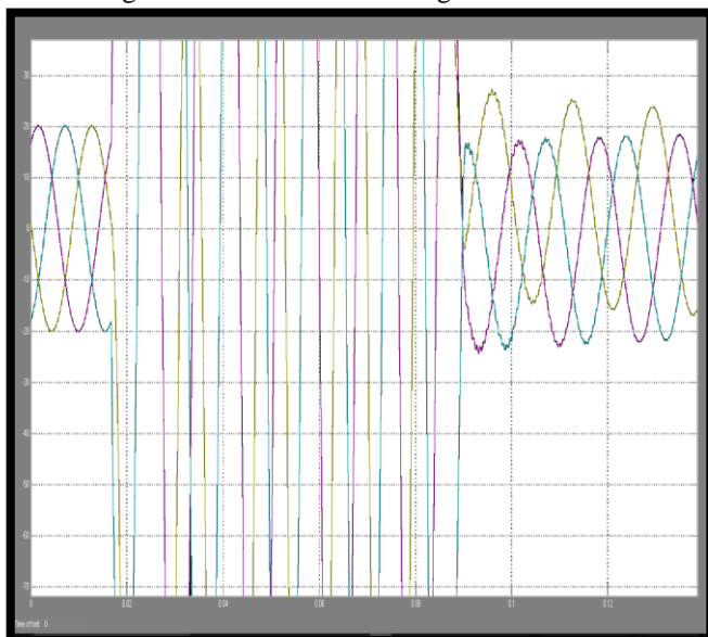
Fig 5.13 Current at B-2 during fault condition with Zoom Scale
