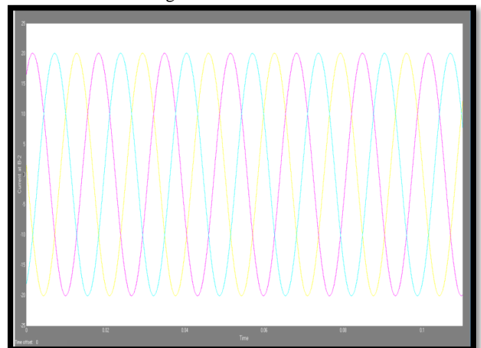
Fig 5.6- Current at B-2
