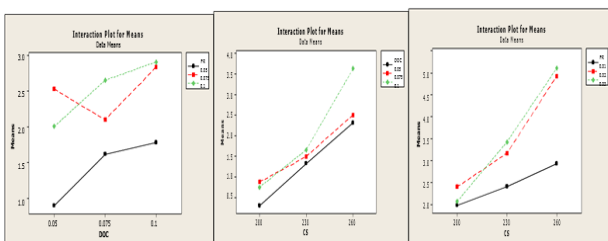
Figure 8. Interaction plot between depth of vibration and feed rate for Production Line vibration in axial direction.
