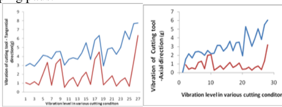
Figure 1 & 2: Displays the comparison of vibration of running. The upper curve shows vibration signal without damping and lower curve is with damping.
