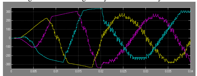
Figure 9. AC Voltage output of Inverter
