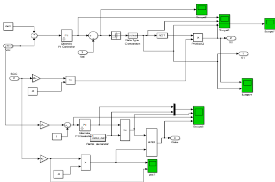
Figure 6. Battery Electrolyze Controller
