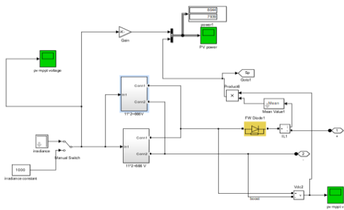
Figure 5. Detailed internal circuit diagram of PV array in Simulink
