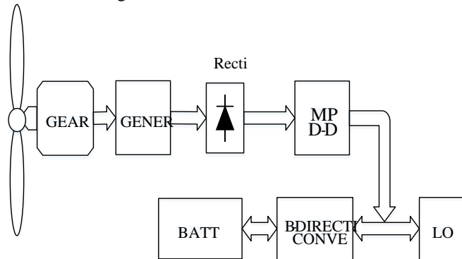
Figure. 2 Overall Block diagram of wind energy system Battery is a storage device which stores the excess power generated and uses it to supply the load in addition to the generators when power is required. Both PV and wind energy systems (described in the previous chapters) are integrated i.e. connected to a common DC bus of constant voltage and the battery bank is also connected to the DC bus. Any power transfer whether from generator to battery bank or generator to load or from the battery bank to the load takes place via this constant voltage DC bus. As the power flow associated with the battery is not uni-directional, a bidirectional converter is needed to charge and/or discharge the battery in case of excess and/or deficit of power respectively.
