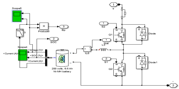
Figure 7. PV system connected with Battery and DC-DC converter
