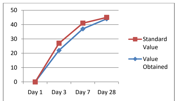
Graph of Compressive Strength Vs Time
