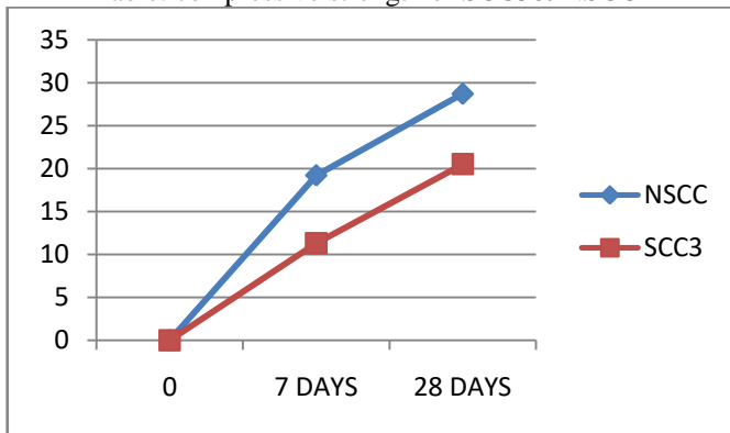
Graph: Compressive strength of SCC3& NSCC
