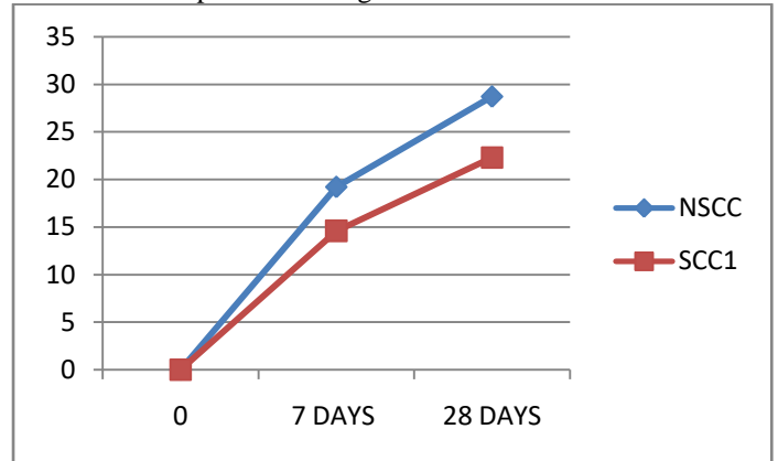
Graph: compressive strength result of SCC1 and NSCC
