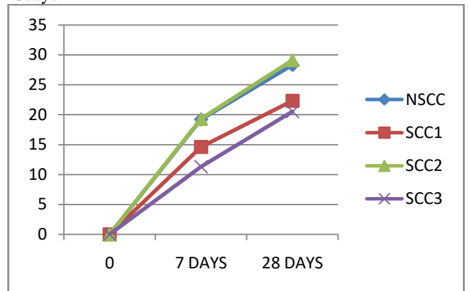
Graph: compressive strength of all mixes
