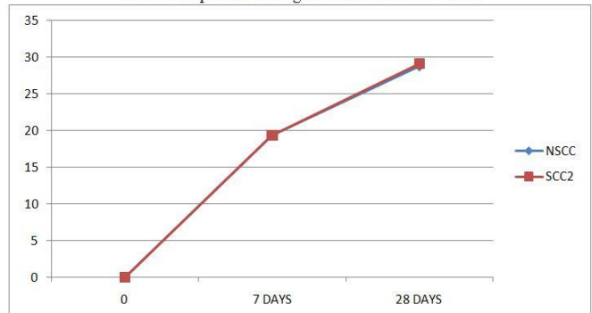
Graph: compressive strength result of SCC2
