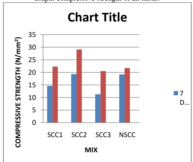
Graph: compressive strength at different ages
