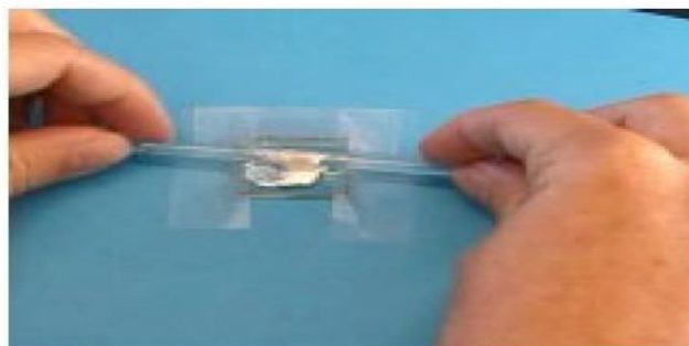
Fig. 7 The titanium dioxide paste and spread using a glass rod
