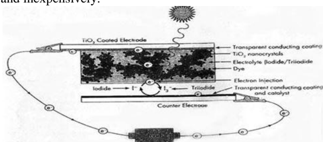
Fig. 3. Nano crystalline dye sensitized solar cell
