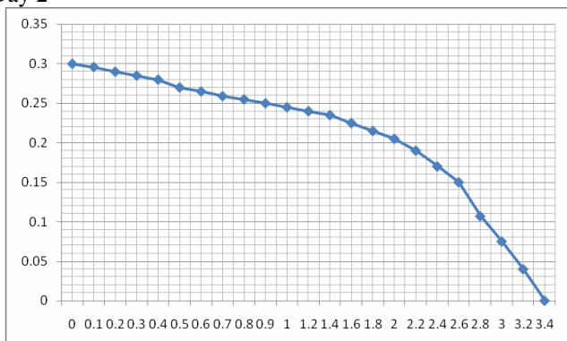
Fig. 14 Graph showing between current and voltage day two
