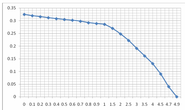
Fig. 13 Graph showing between current and voltage The output characteristics of solar cell on day one are shown in fig. 13. The graph shown & between current & voltage. The current is on x-axis and voltage is y-axis calculated the value of I_{max} and V_{max} using the graphs. The results are shown in table 3.
