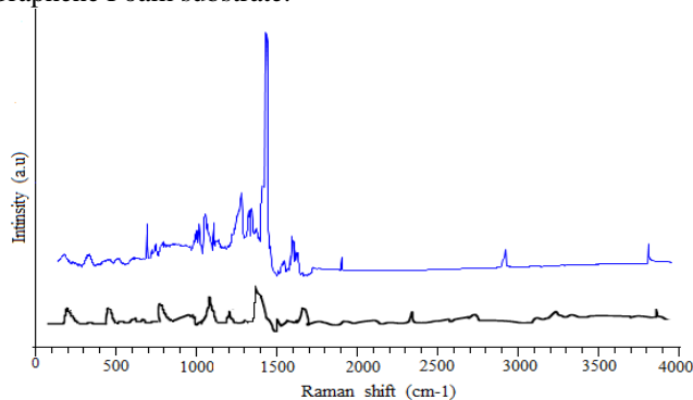
Figure 5. Comparison of SERS intensity of 1\mu\text{M} MB on different SERS including Graphene Foam (black color) and AuNPs/GF (blue color).
