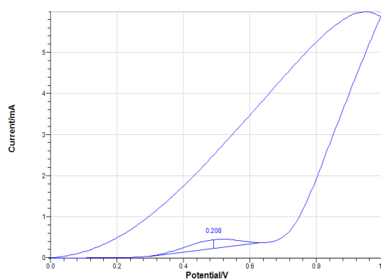
Figure 3. Shows the cyclic voltammetry of hydrogen peroxide at scan rate in 50 mV/s.
