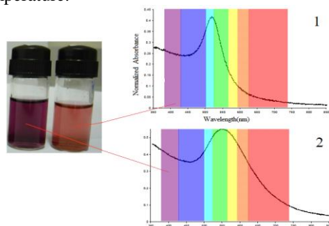
Figure 1. UV-Vis absorption spectrum of gold nanoparticles.
