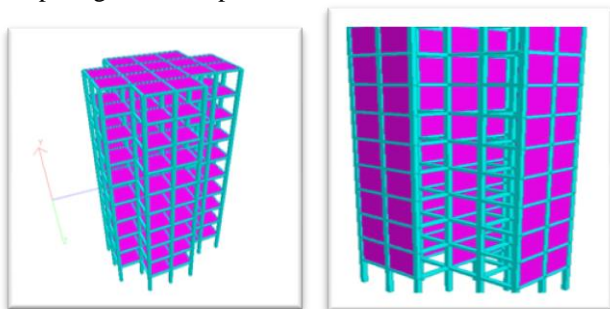
FIG.1: STRUCTURE WITHOUT SHEAR WALL FIG.2: STRUCTURE WITH SHEAR WALL
