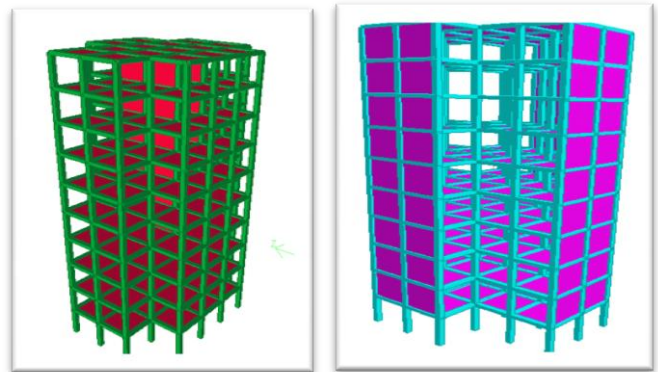
FIG.3: STRUCTURE WITH INNER SHEAR WALL FIG.4: STRUCTURE WITH OUTER SHEAR WALL
