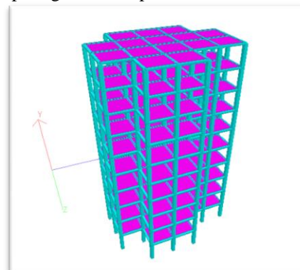
FIG.1: STRUCTURE WITHOUT SHEAR WALL
