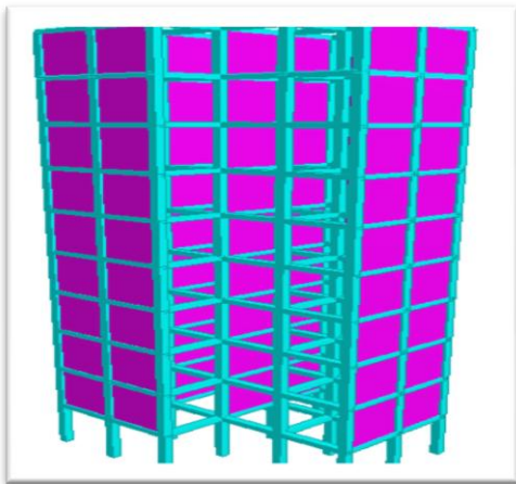
FIG.2: STRUCTURE WITH SHEAR WALL
