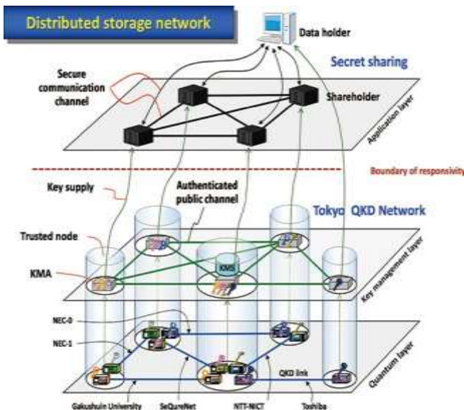
Figure 4: A secret sharing storage network using QKD.
