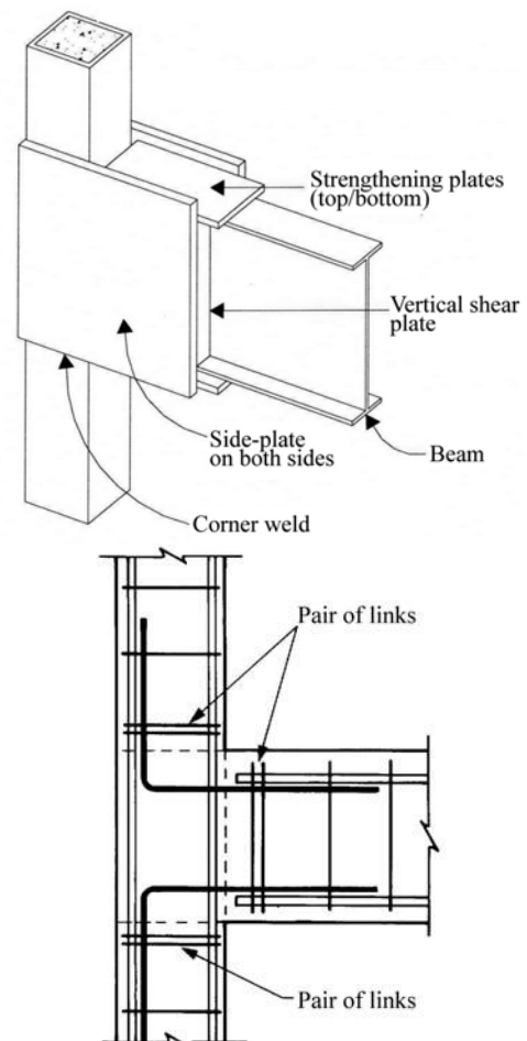
Figure 8. Enhanced beam-to-column connection details for steelwork [7] and reinforced concrete [3]
