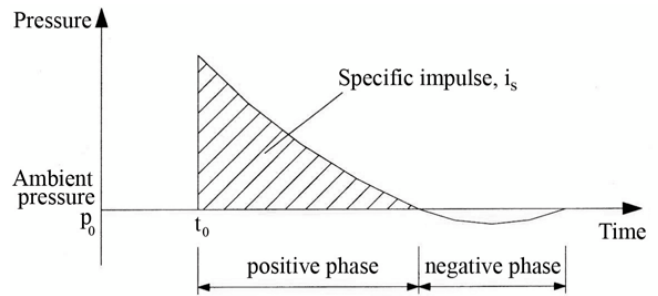
Figure 4. Blast wave pressures plotted against time As a rough approximation, 1kg of explosive produces about 1m 3 of gas. As this gas expands, its act on the air surrounding the source of the explosion causes it to move and increase in pressure. The movement of the displaced air may affect nearby objects and cause damage. Except for a confinement case, the effects of the dynamic pressure diminish rapidly with distance from source.
