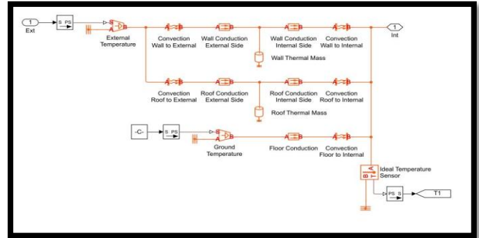
Fig 10- Thermal Effect control subsystem
