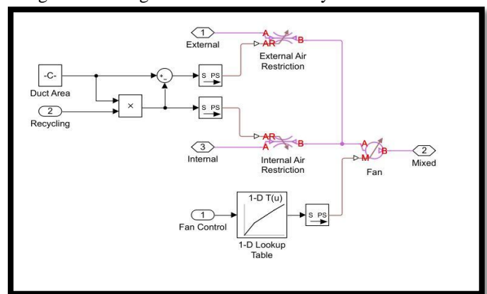
Fig 11- Ventilation Control subsystem
