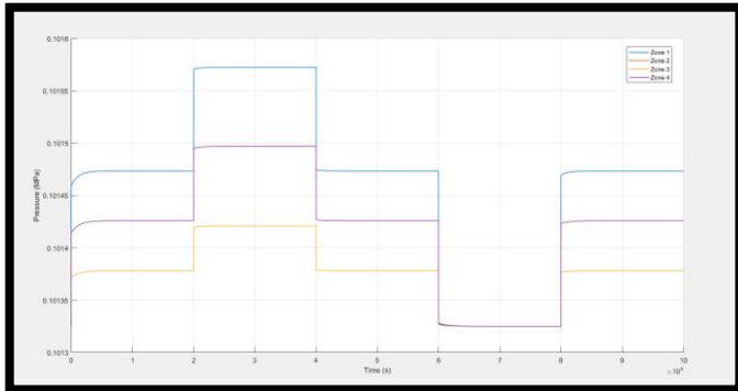
Fig 15- Pressure output parameters of the building structures
