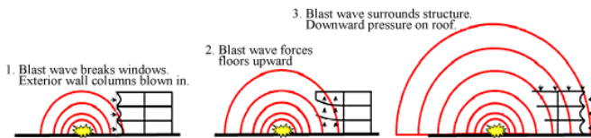
Figure 7. Sequence of air-blast effects [5]
