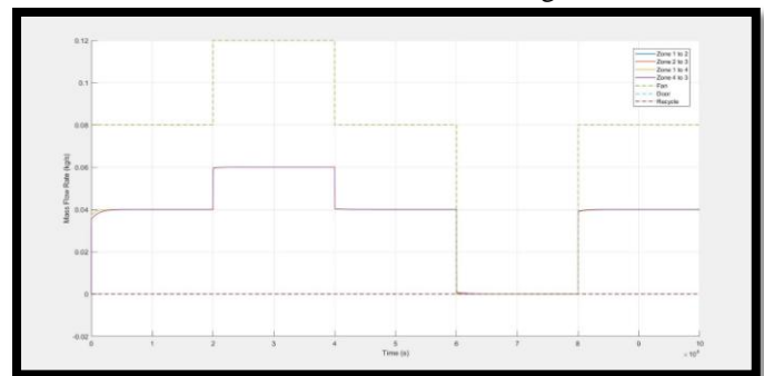
Fig 12- Building Mass flow controlling subsystem
