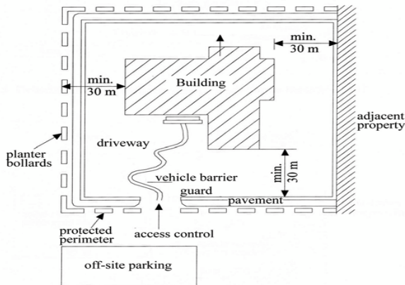
Figure 5. Schematic layout of site for protection against bombs [8]
