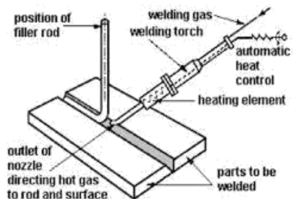
Schematic of hot gas welding showing correct position of torch and filler rod
