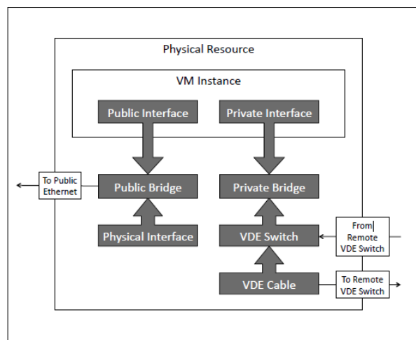
Figure 2: INSTANCE MANAGER
