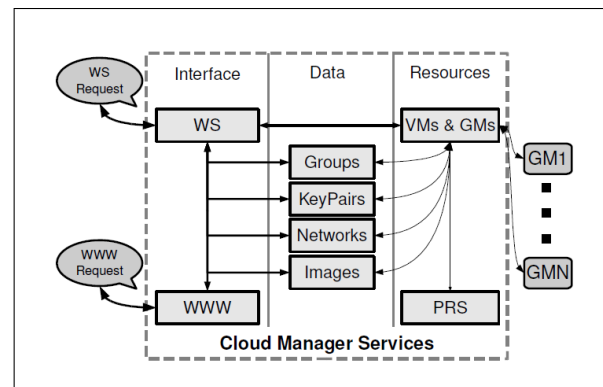
Figure 3: CLOUD MANAGER
