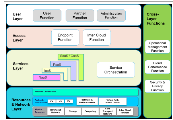
Figure 1: key functions of a cloud management system
