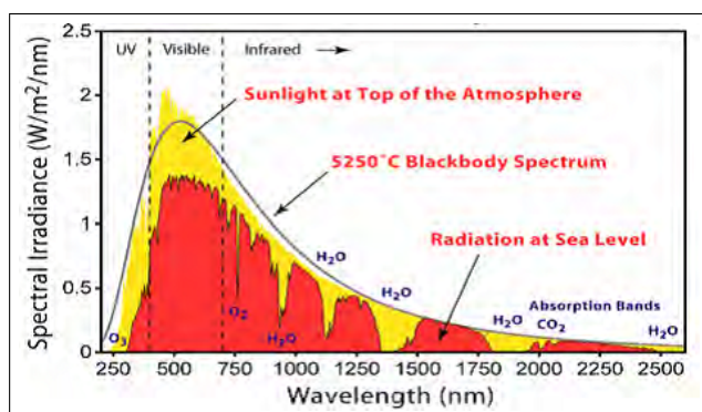
Figure 7: Spectral irradiance of the Sun
