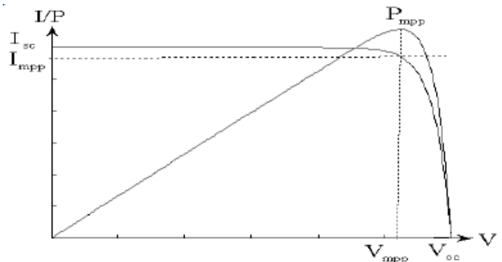
Figure 1: I-V and P-V characteristics of photovoltaic cell
