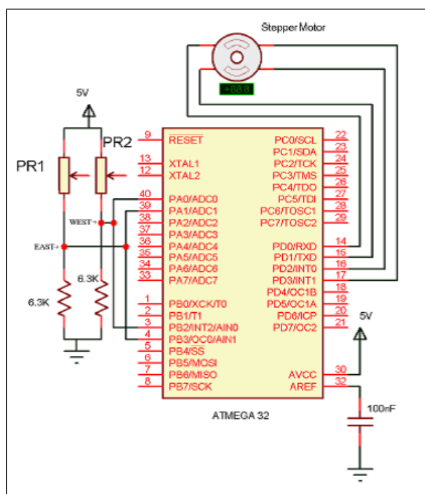
Figure 3: Schematic of solar tracker circuitry
