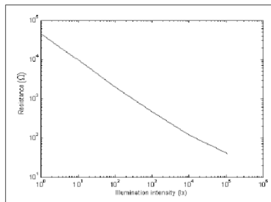
Figure 2: Represents the resistance value of the photo resistor with the illumination of light
