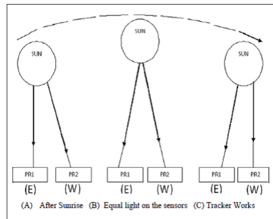
Figure 6: Solar tracker working mechanism
