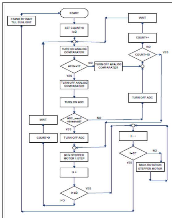
Figure 5: Operational flow chart of the solar tracker
