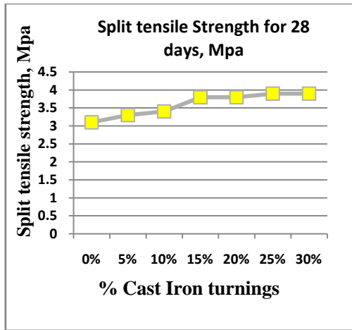
Figure 8. Split tensile strength for 28 days
