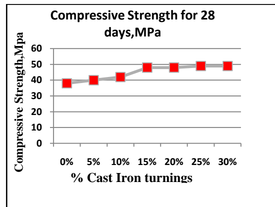
Figure 4. Compressive strength for 28 days
