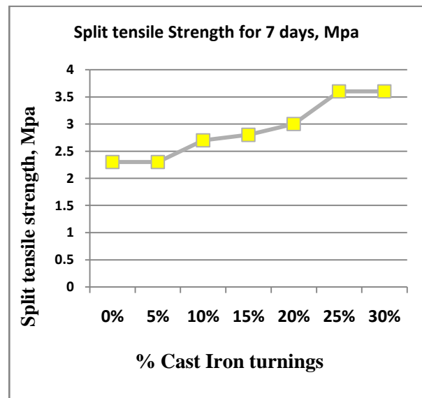
Figure 7. Split tensile strength for 7 days
