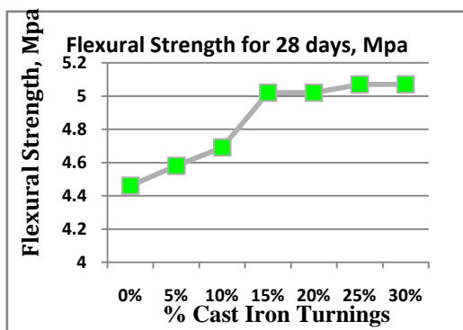
Figure 6. Flexural strength for 28 days
