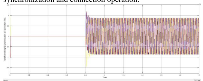
Fig 4.11- Grid Current in grid synchronization and connection using proposed method
