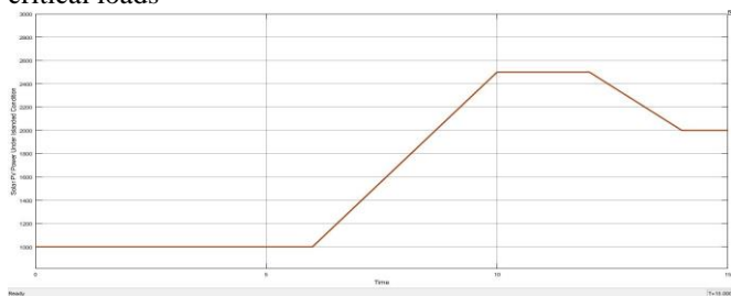
Fig 4.7- Solar PV Power under Isolated Mode in MW
