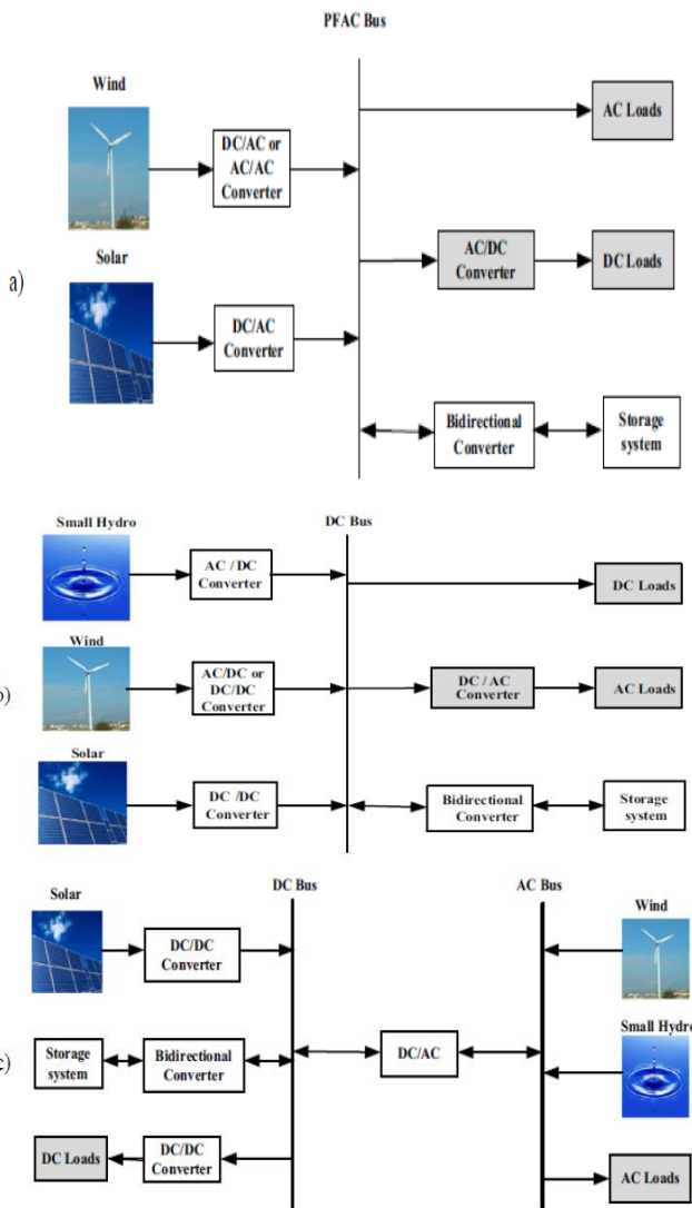
Figure 2.1 Microgrid configurations: a) AC coupled b) DC coupled c) Hybrid coupled
