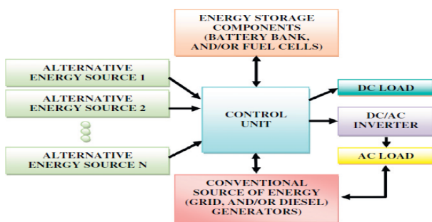
Figure 1.1 General structure of a microgrid system
