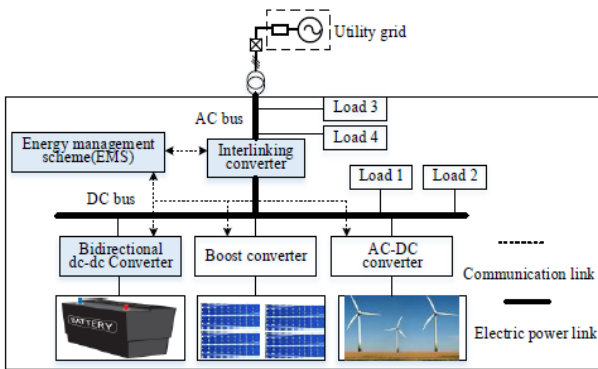
Fig. 3.1 a microgrid with multiples energy sources and converters
