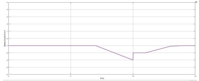
Fig 4.8- Battery Current under Isolated Mode in A High wind and irradiation and light load
