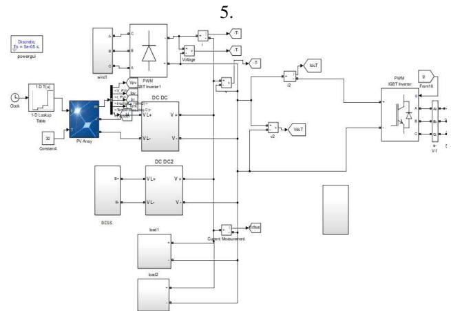
Fig 4.1- Matlab Simulation of A microgrid with multiples energy sources and converters
