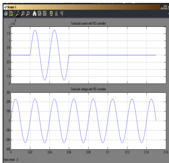
Fig 2 :- total fault current during fault with PID control
