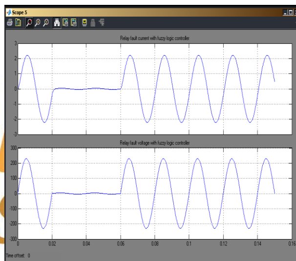
Fig 3 :- relay fault current during fault with fuzzy logic control
