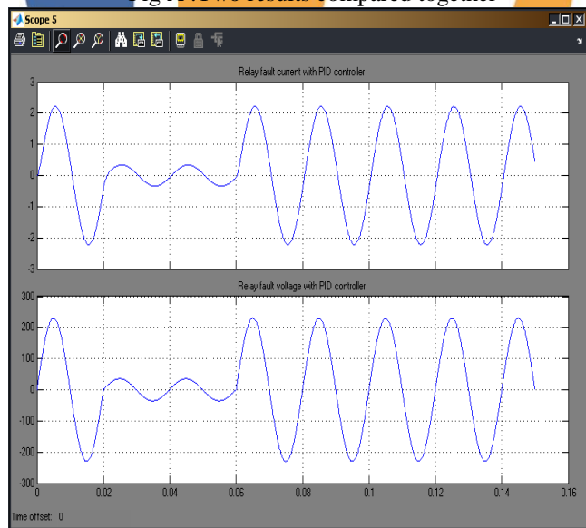
Fig 1 :- relay fault current during fault with PID control
