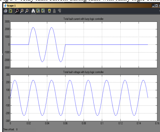
Fig 4 :- total fault current during fault with fuzzy logic control
