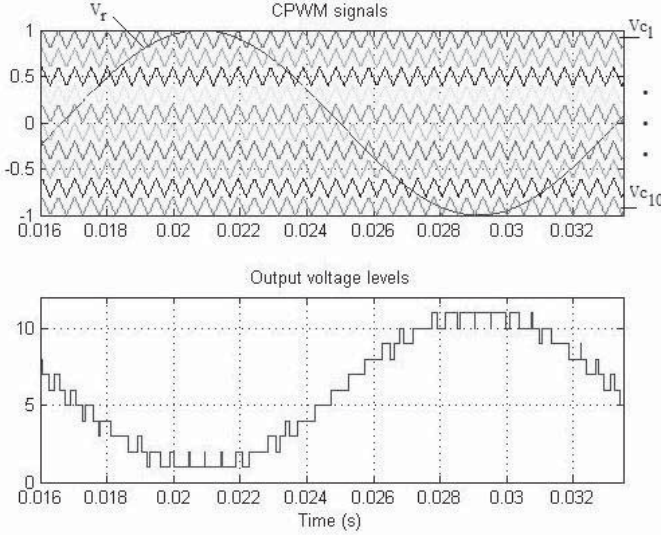
Fig. 4. CPWM waveforms for an 07-level MMC inverter, and the generated output voltage levels.
