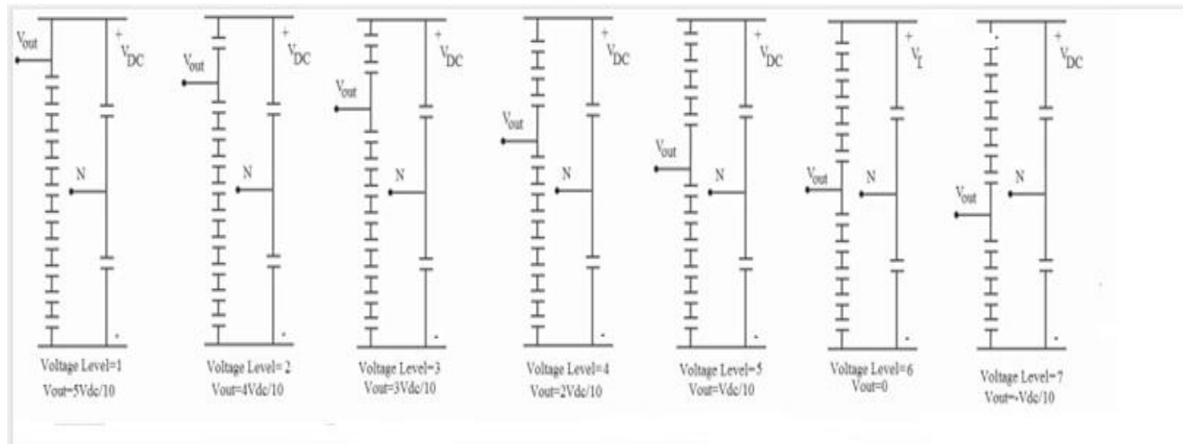
Fig. 5. Selection of SMs' capacitors for different voltage levels.
