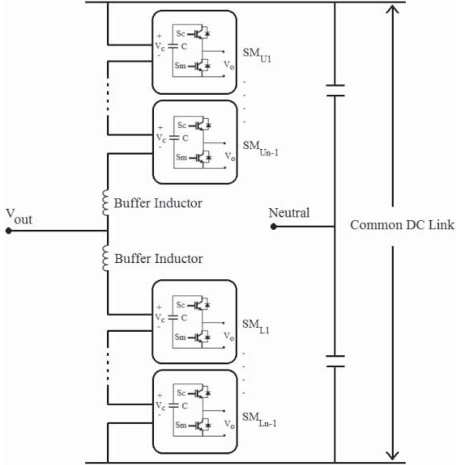
Fig. 2. Structure of a single-phase MMC inverter structure.
