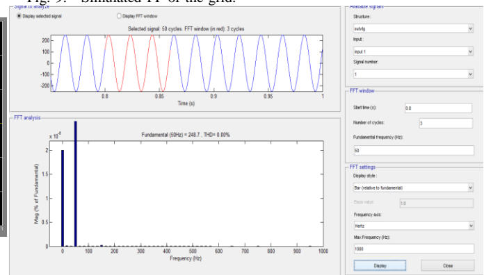
Fig. 10. Simulated delta and modulation index of the 07-level inverter.
