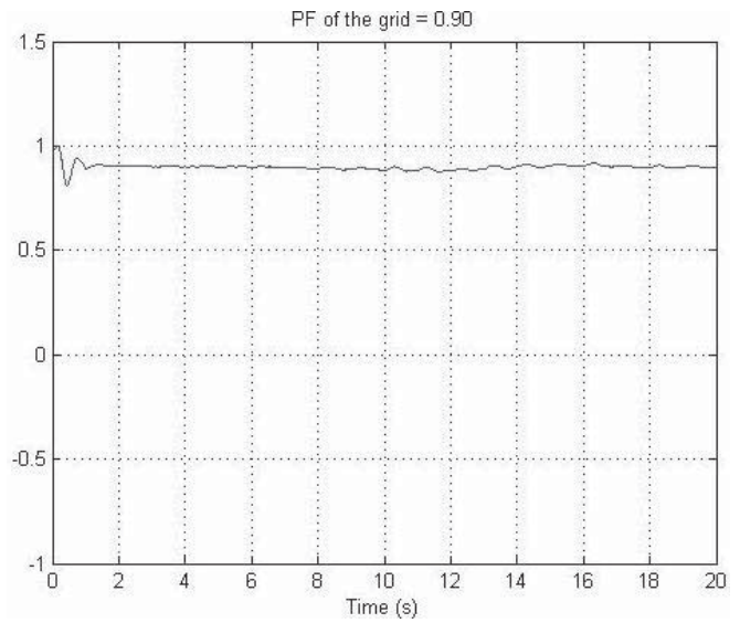
Fig. 9. Simulated PF of the grid.
