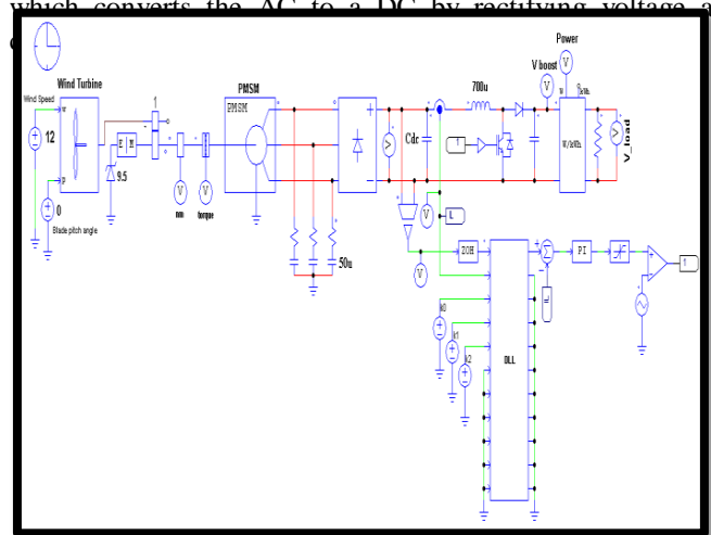
Fig. 1 Wind energy Energy
